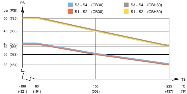
CB30 – PED approval pressure/temperature graph
