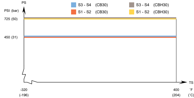
CB30 – UL approval pressure/temperature graph
