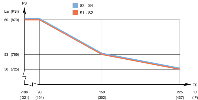
CBP30 – PED approval pressure/temperature graph
